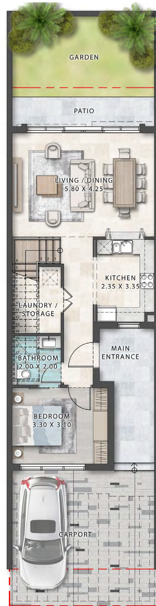
GROUND FLOOR
