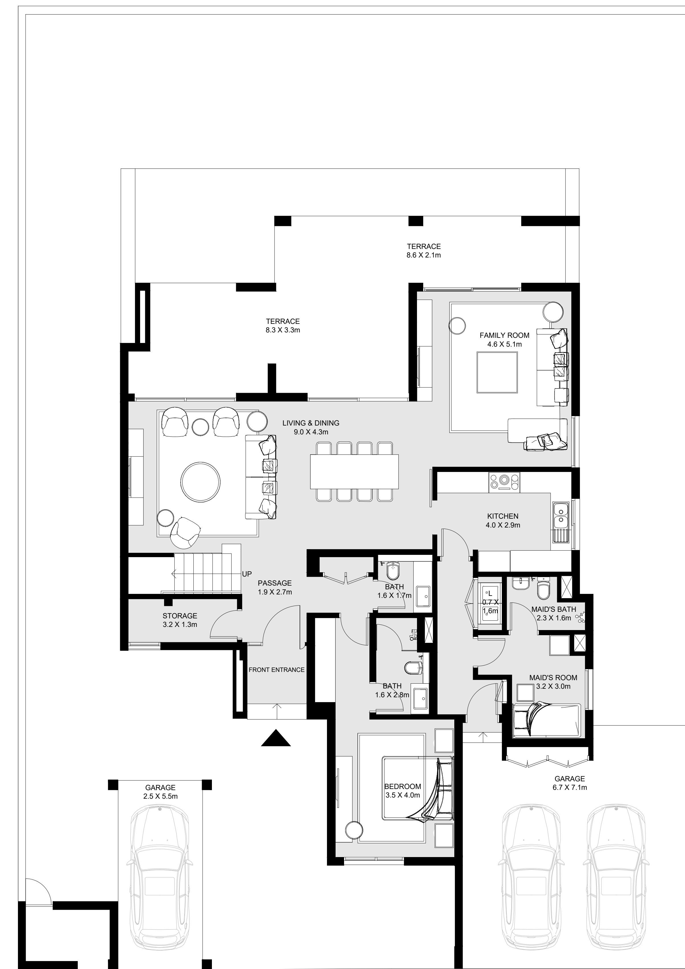
GROUND FLOOR
