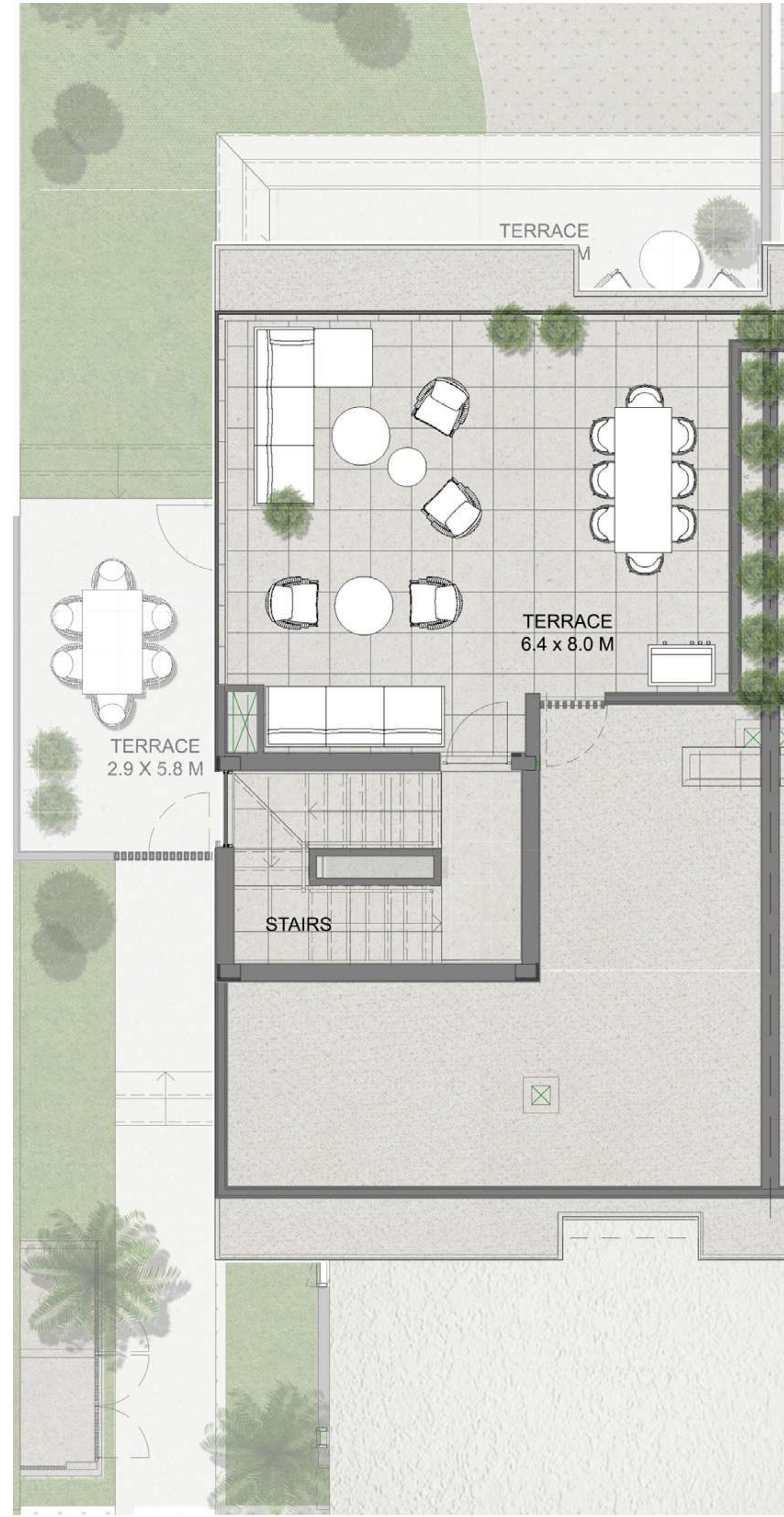
Roof Terrace
