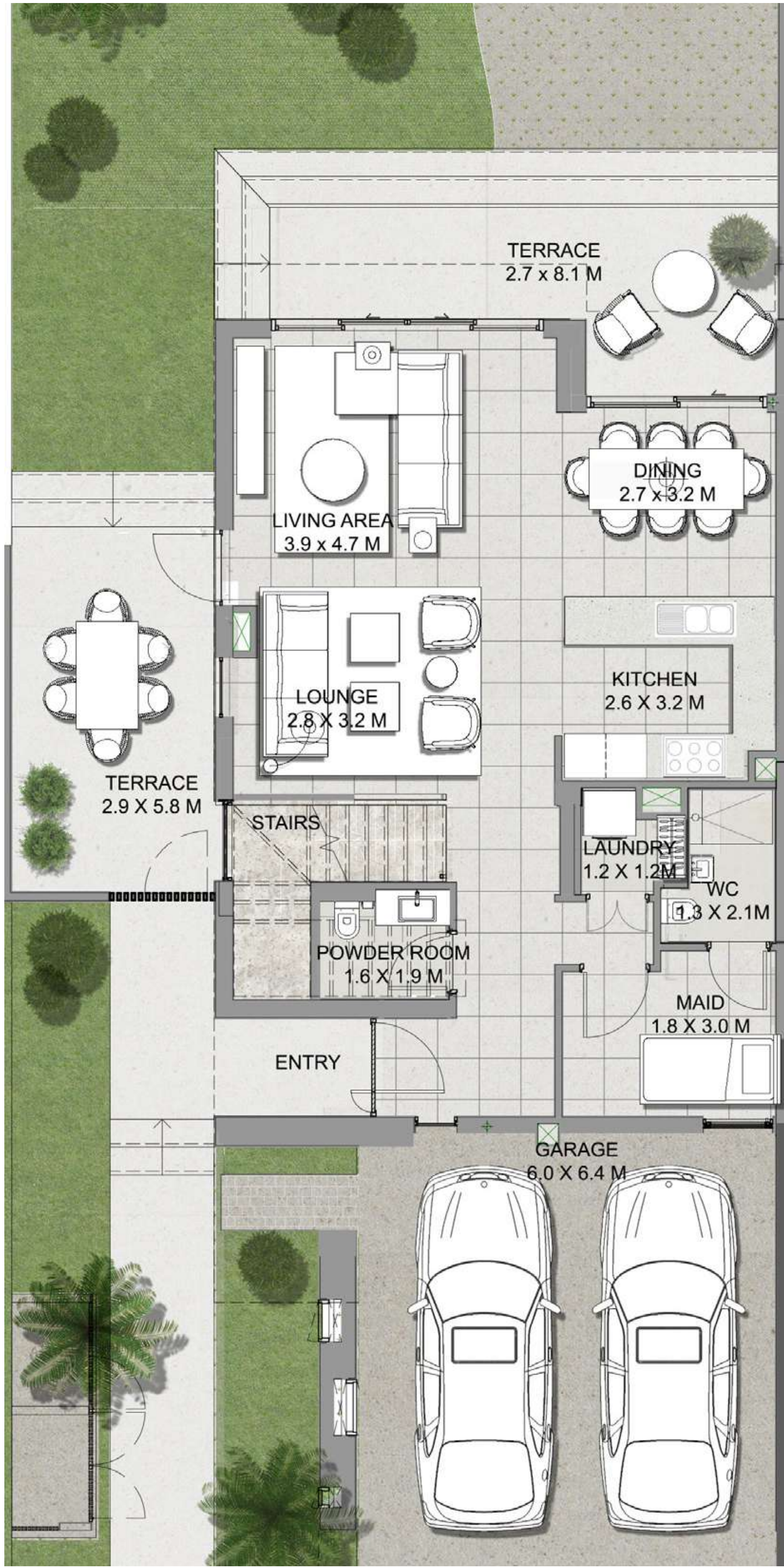
Ground floor
