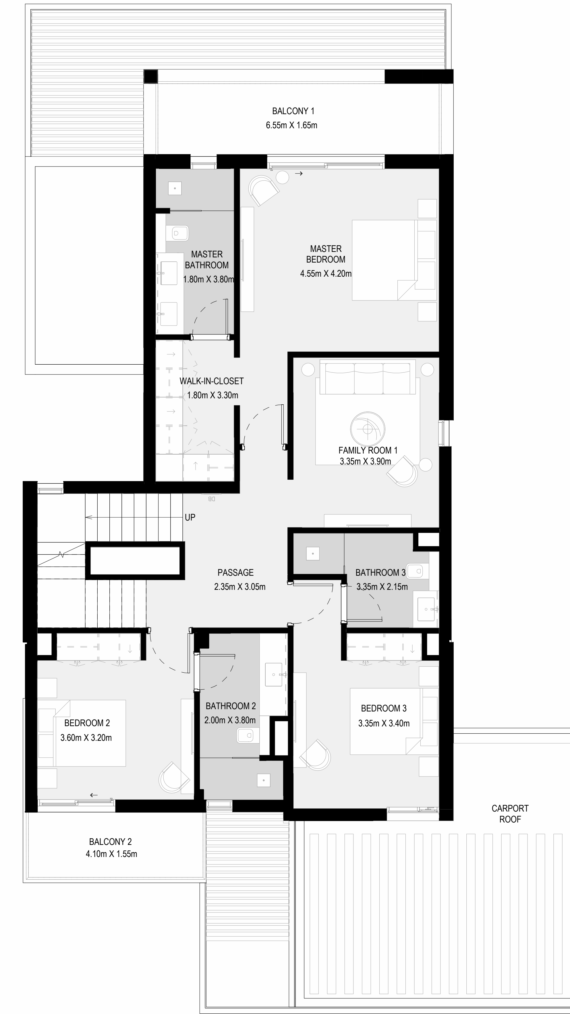
FIRST FLOOR
