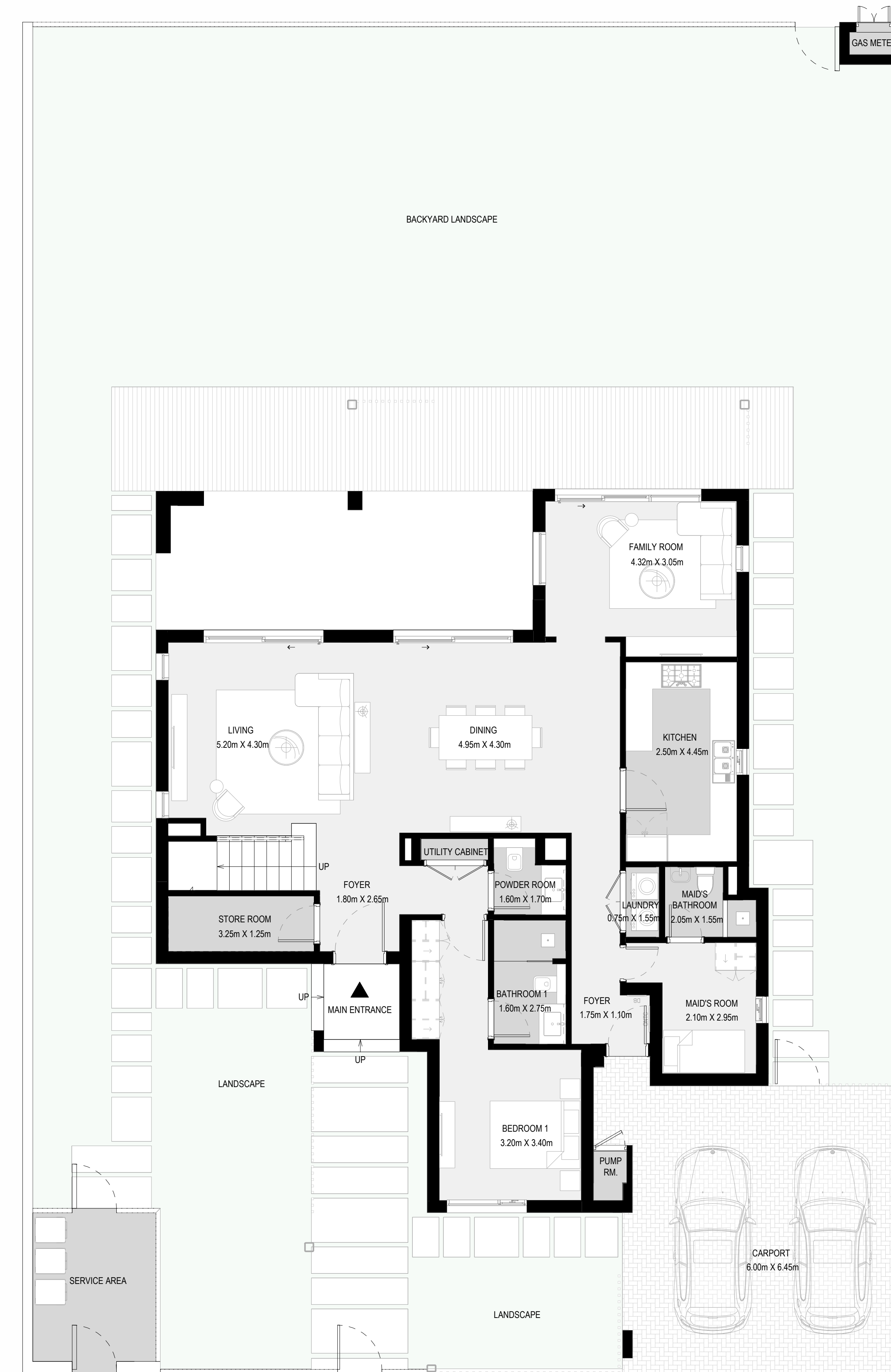
GROUND FLOOR
