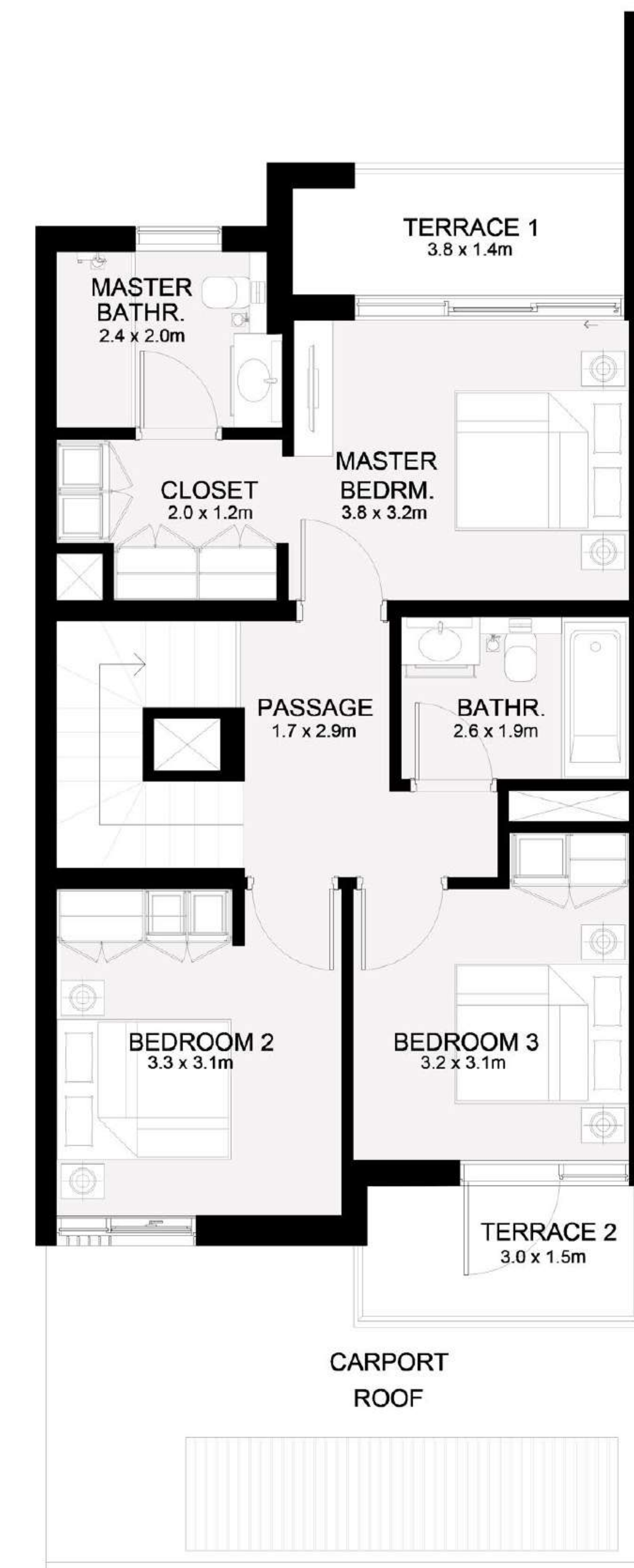
FIRST FLOOR
