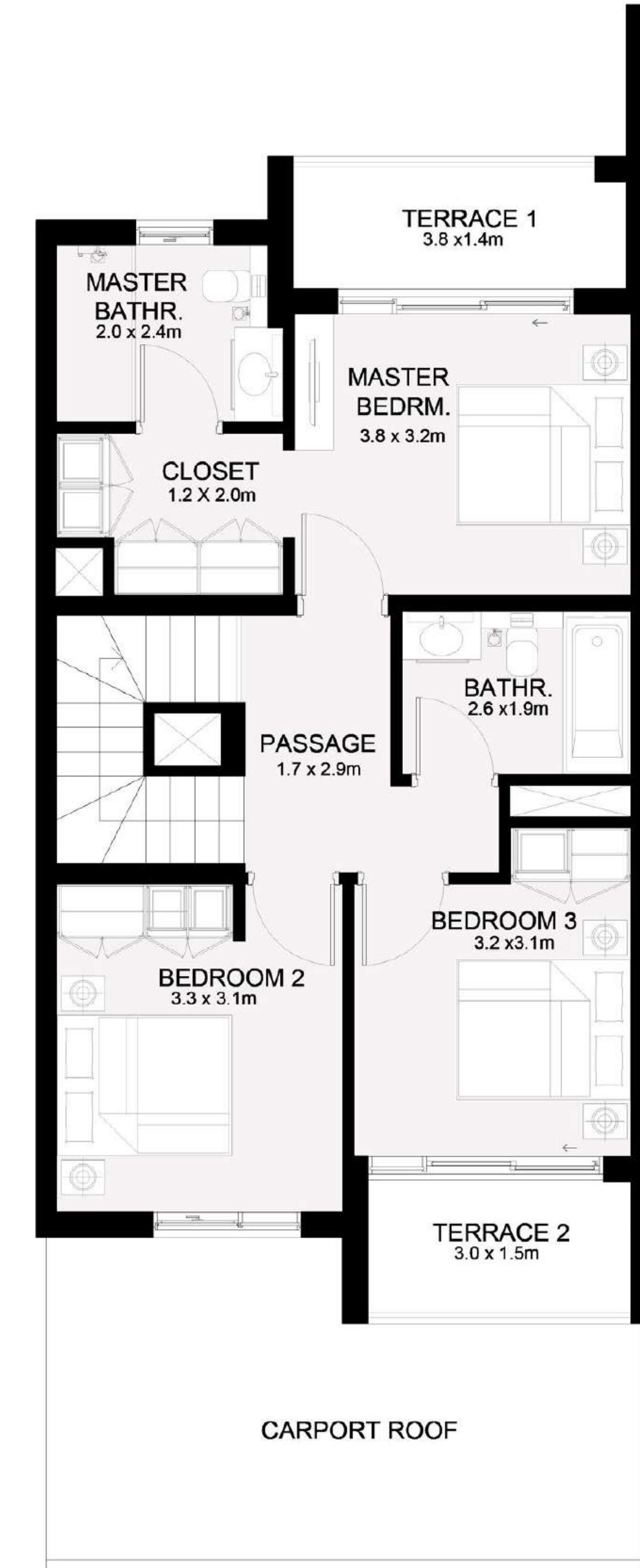
FIRST FLOOR
