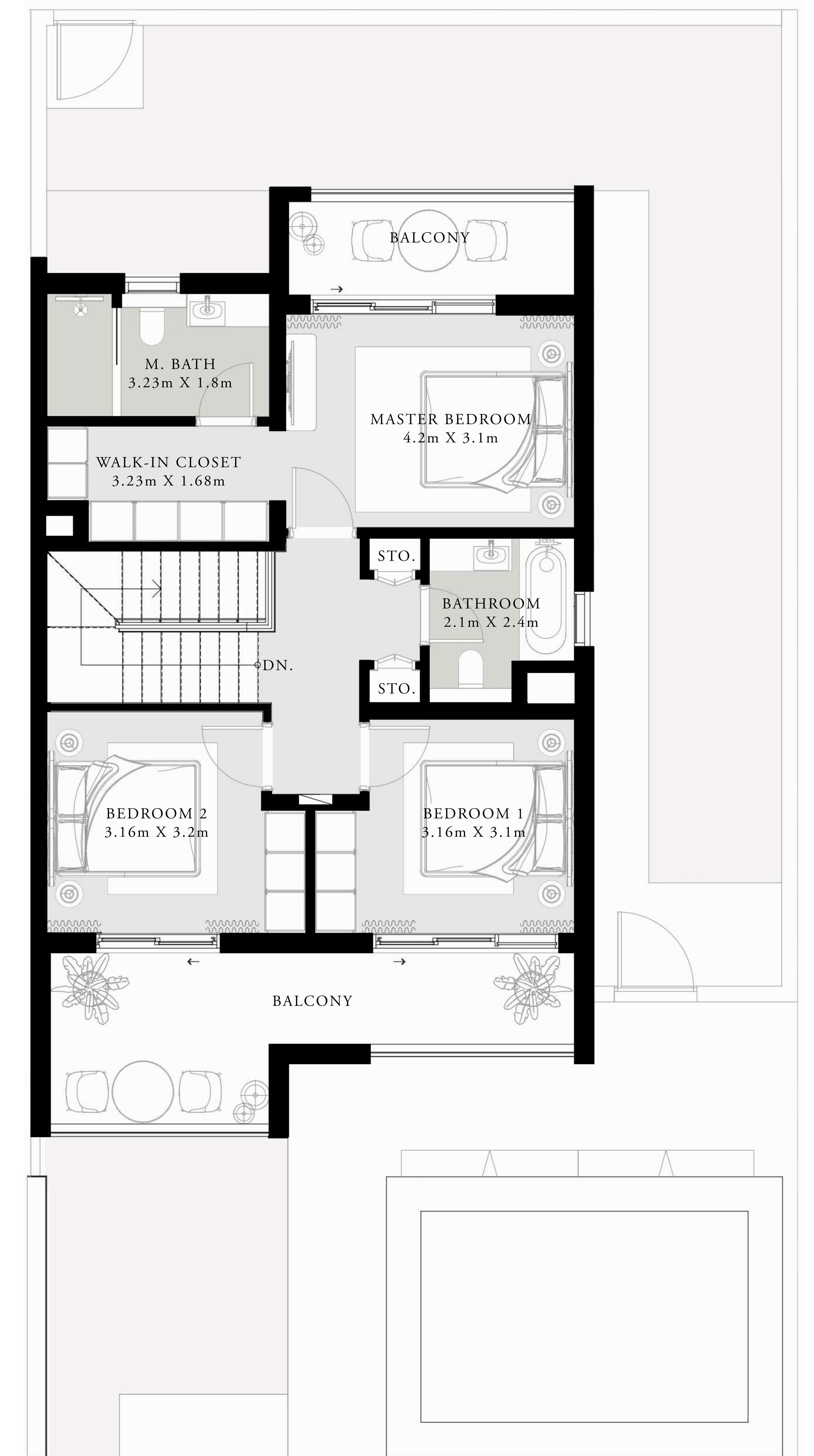
FIRST FLOOR
