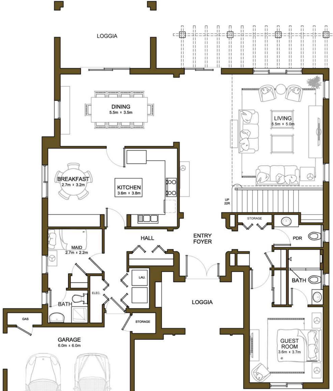
GROUND FLOOR
